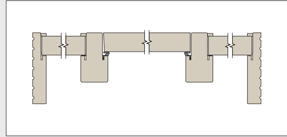
Single Rabbet Frame with 4 5/16\" Uniframe Mull Posts
