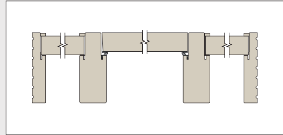
Single Rabbet Frame with 6 3/16\" Uniframe Mull Posts
