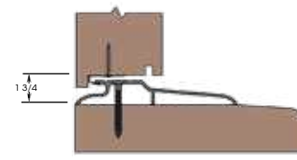
Interlocking Sill
