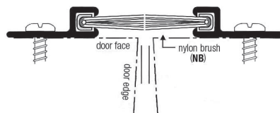
Threshold ADA Compliant 1/2" x 5" x 3 ft., 4 ft., 8 ft., 6 ft. 5SDLTHRESH30, 5SDLTHRESH40, 5SDLTHRESH60
