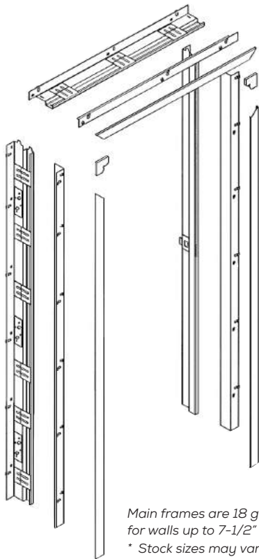
Universal Application (Adjustable Split Frame - Interior & Exterior Application)
