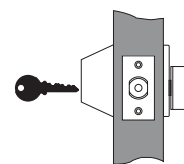
Single Cylinder Deadbolt D212 (edge view) Outside locked by key in outside. Inside locked by turn latch.
