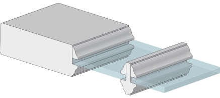
Narrow Reverse Roman Ogee (OG) Sash*
