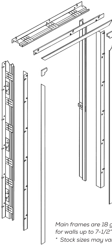
Universal Application (Adjustable Split Frame - Interior & Exterior Application)
