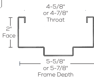
Drywall Application (Interior Application Only)
