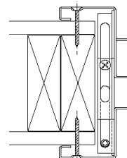
Adjustable Application (Interior & Exterior Application)
