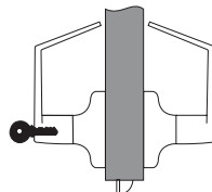
Classroom 4608LN Outside locked by key in outside lever. Inside lever always active.
