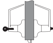
Entry 4607LN Outside lever locked by inside push button. Inside lever always active. Unlocked by turning inside lever or emergency key in exterior.
