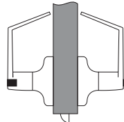
Privacy 4602LN Outside lever locked by inside push button. Inside lever always active. Unlocked by turning inside lever or emergency key in exterior.
