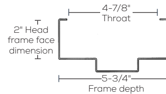
Universal Application (Interior & Exterior Application)
